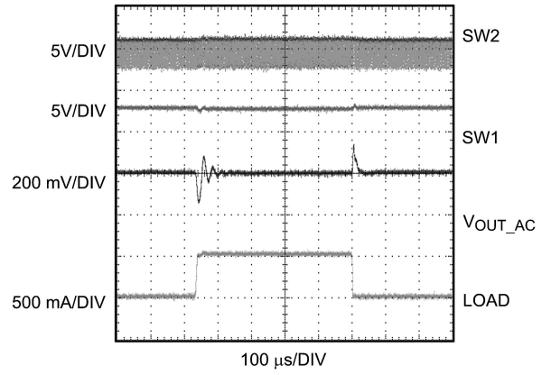
Load Transient in Boost Operation (Forced PWM Mode)
