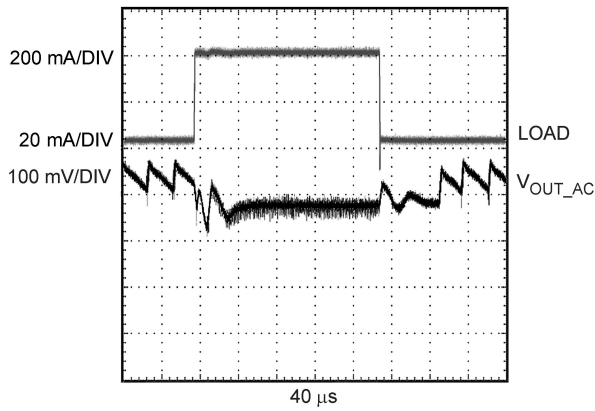
Load Transient in Buck-Boost Mode (Auto Mode) V_{IN} = 3.6V, V_{OUT} = 3.3V, \text{Load} = 50-150mA
