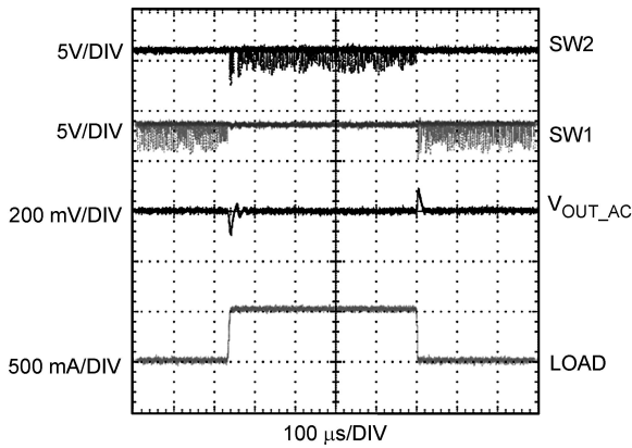
Load Transient in Buck-Boost Operation (Forced PWM Mode)
