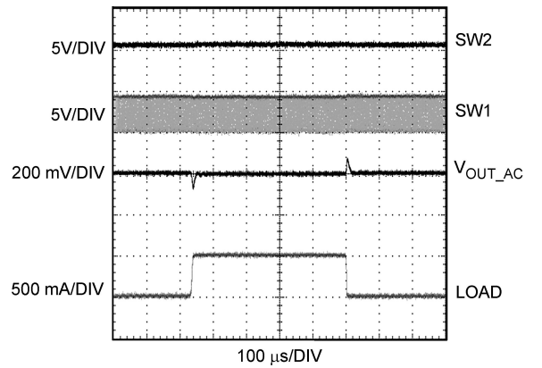
Load Transient in Buck Mode (Forced PWM Mode)
